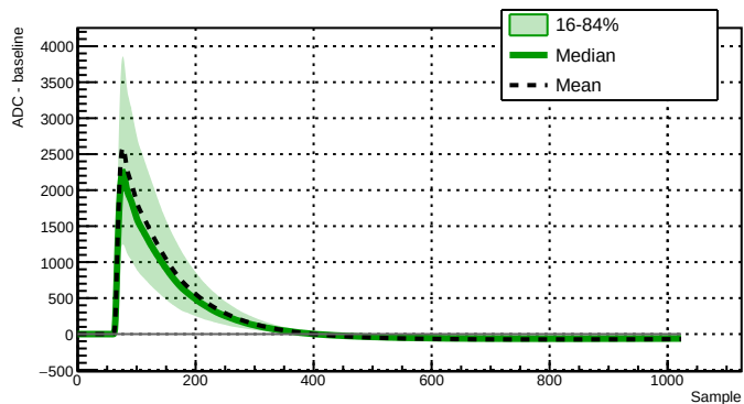
Run 039528 - Channel 2060 - 5633 waveforms
