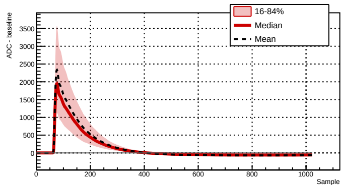
Run 039528 - Channel 2061 - 3703 waveforms
