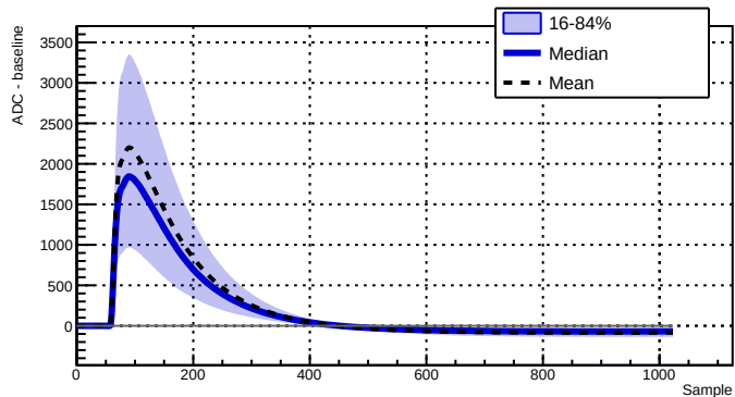
Run 039528 - Channel 2050 - 8182 waveforms
