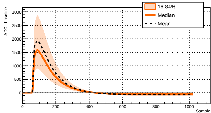
Run 039528 - Channel 2051 - 5779 waveforms
