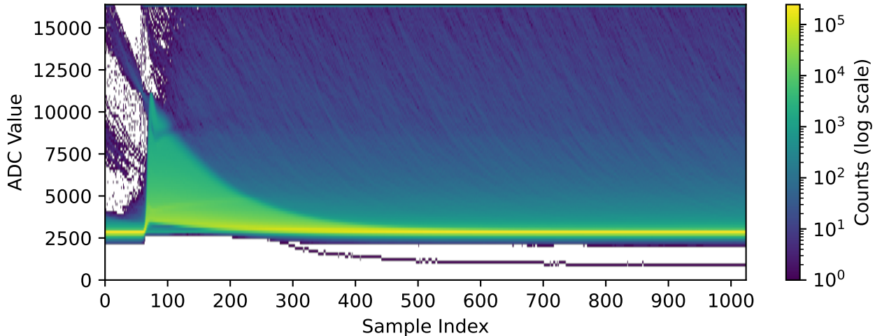
Channel 1011 (n=283440 waveforms)
