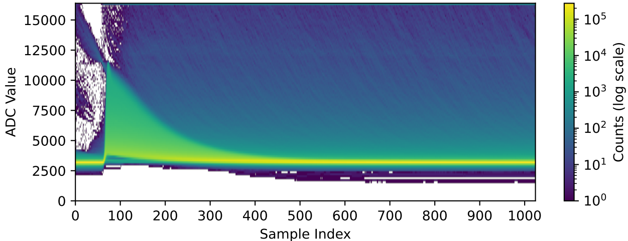
Channel 1021 (n=328434 waveforms)
