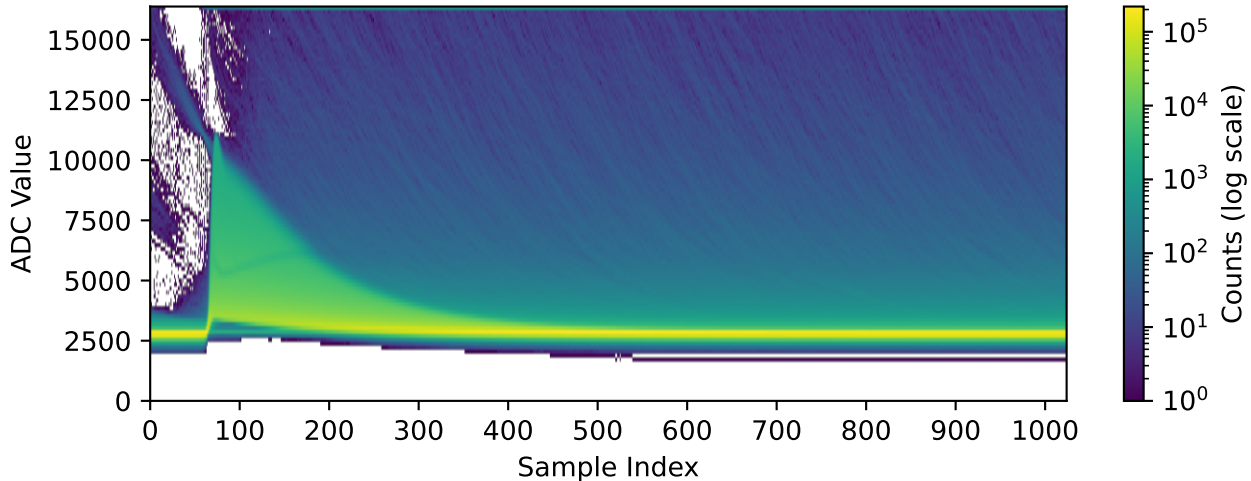
Channel 1040 (n=311702 waveforms)
