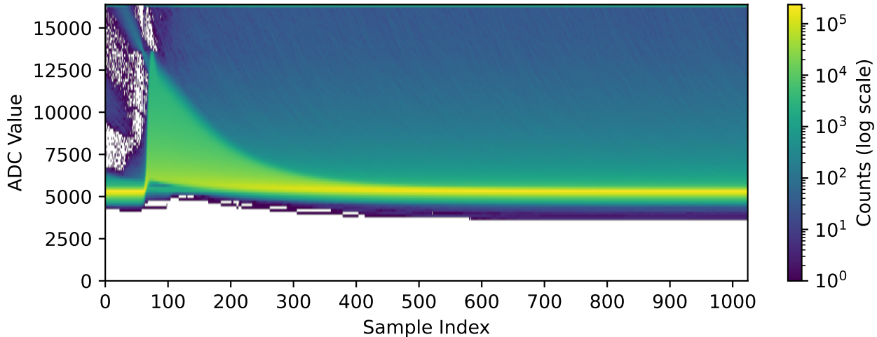
Channel 1051 (n=389436 waveforms)
