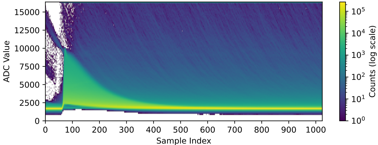
Channel 1060 (n=312547 waveforms)
