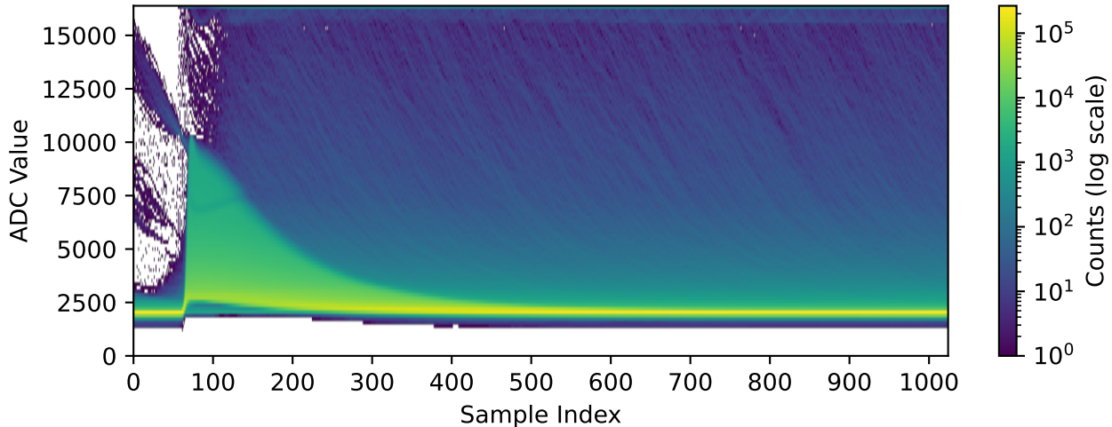
Channel 1080 (n=301913 waveforms)
