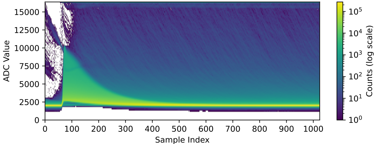
Channel 1080 (n=305514 waveforms)
