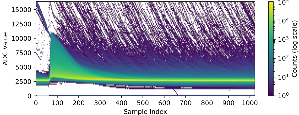
Channel 2021 (n=127214 waveforms)
