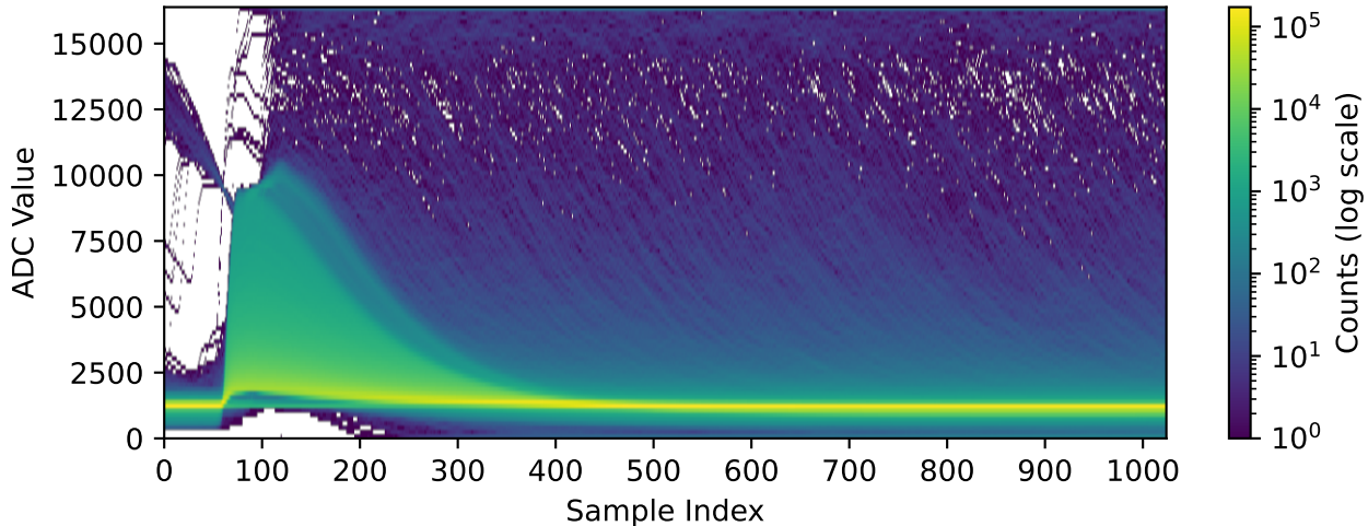
Channel 2051 (n=202240 waveforms)
