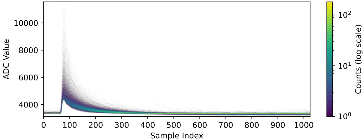
Channel 2070 (n=3504 waveforms)
