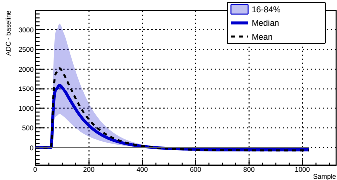
Run 039500 - Channel 2080 - 16582 waveforms
