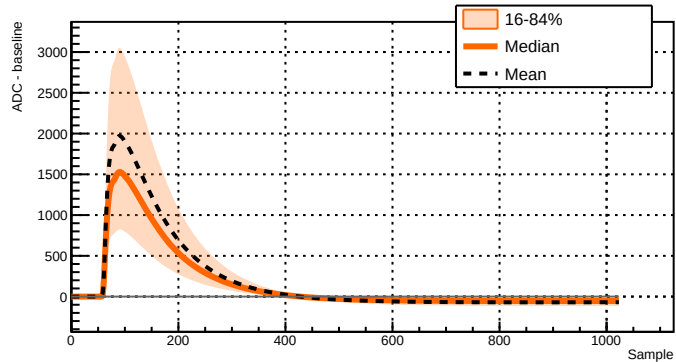
Run 039500 - Channel 2081 - 17000 waveforms
