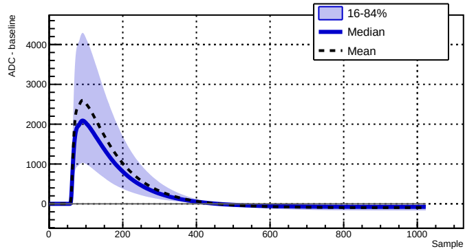
Run 039512 - Channel 2080 - 23204 waveforms
