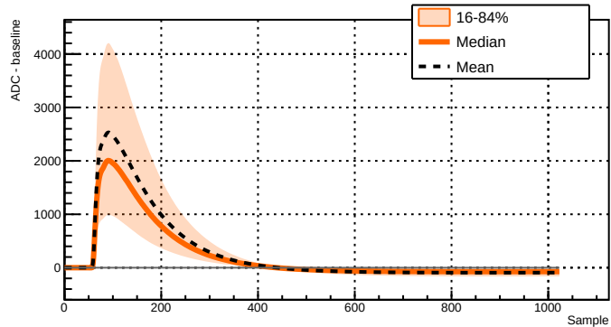
Run 039512 - Channel 2081 - 23597 waveforms
