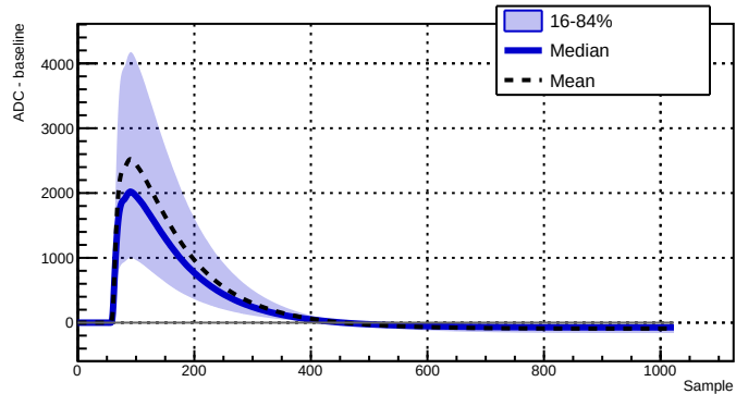
Run 039514 - Channel 2080 - 22354 waveforms
