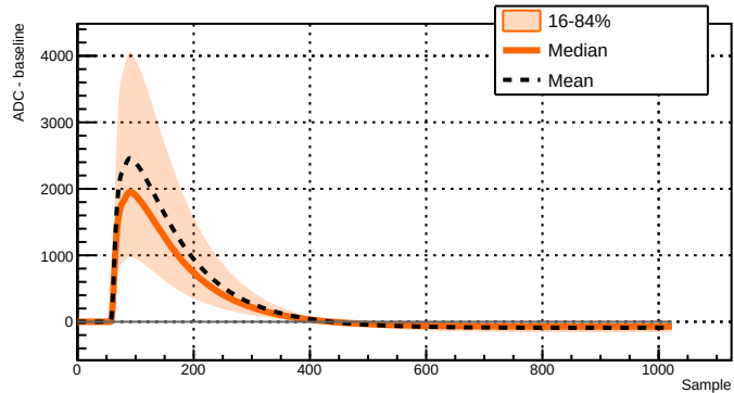
Run 039514 - Channel 2081 - 22661 waveforms
