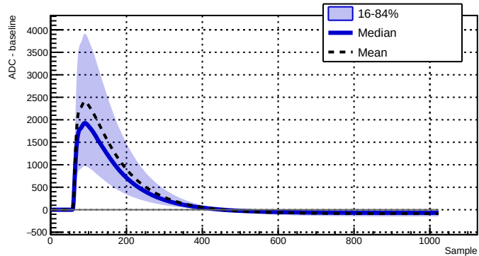
Run 039516 - Channel 2080 - 20465 waveforms
