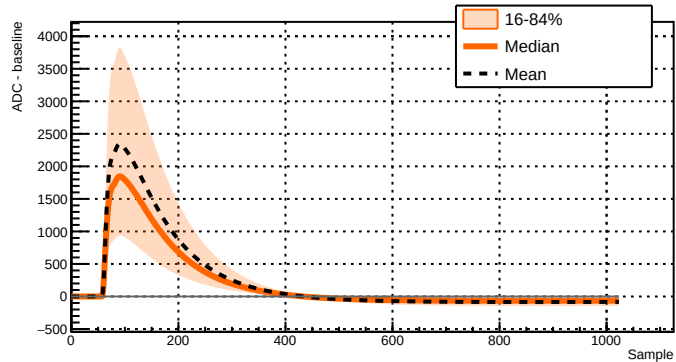
Run 039516 - Channel 2081 - 20743 waveforms
