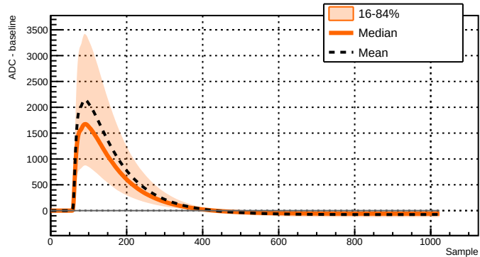
Run 039521 - Channel 2081 - 19065 waveforms
