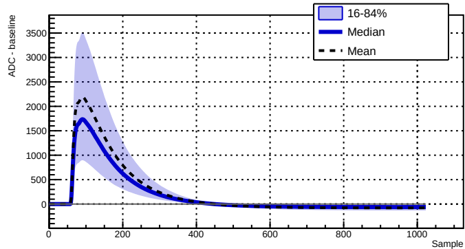
Run 039521 - Channel 2080 - 18742 waveforms
