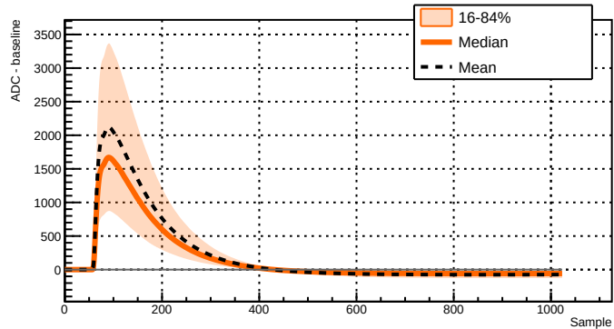
Run 039522 - Channel 2081 - 18966 waveforms
