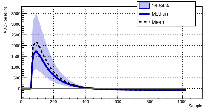
Run 039522 - Channel 2080 - 18484 waveforms
