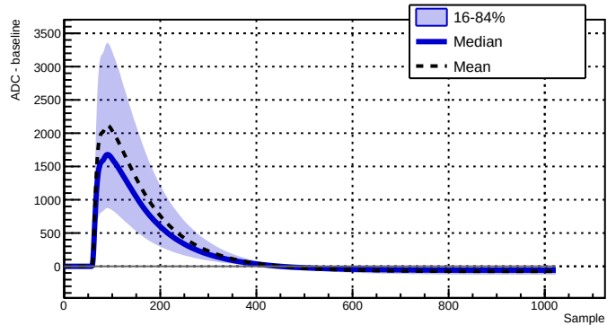
Run 039523 - Channel 2080 - 17862 waveforms
