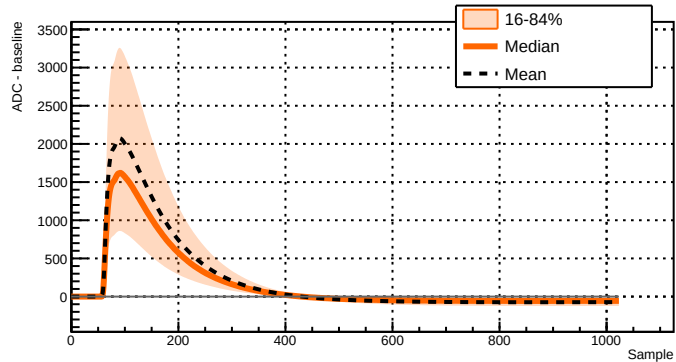
Run 039523 - Channel 2081 - 18293 waveforms
