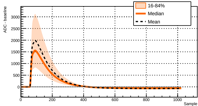
Run 039527 - Channel 2081 - 17165 waveforms
