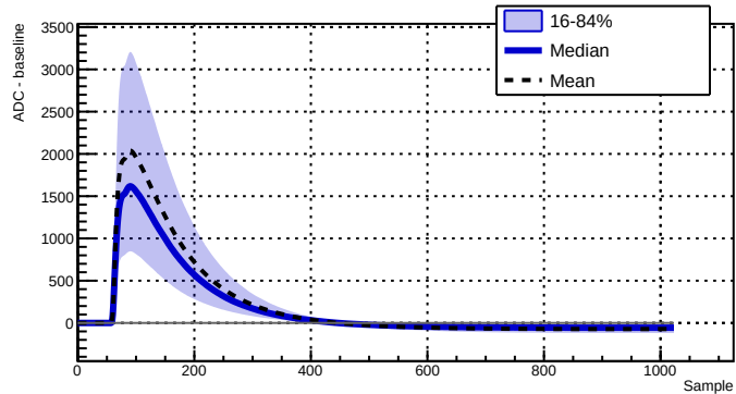
Run 039527 - Channel 2080 - 16770 waveforms
