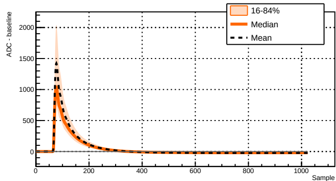
Run 039501 - Channel 2071 - 8633 waveforms
