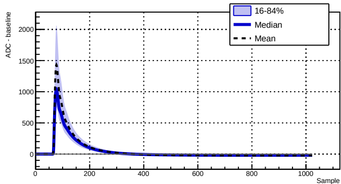
Run 039501 - Channel 2070 - 8976 waveforms
