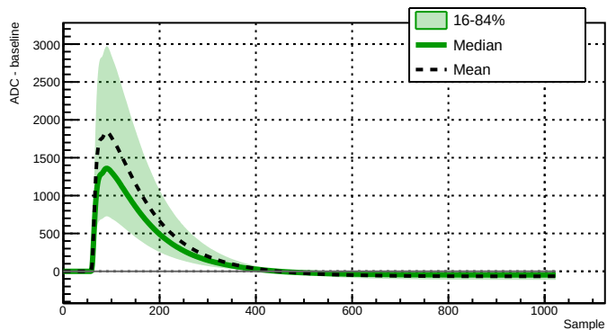
Run 039501 - Channel 2080 - 30706 waveforms
