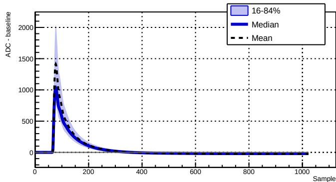
Run 039503 - Channel 2070 - 10138 waveforms
