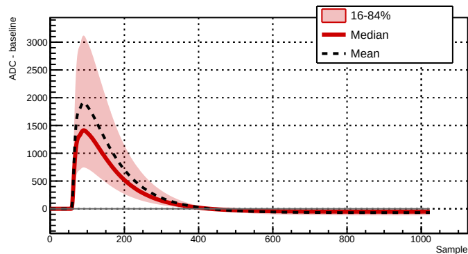
Run 039503 - Channel 2081 - 32524 waveforms
