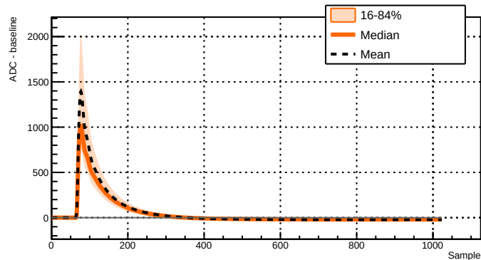
Run 039503 - Channel 2071 - 9884 waveforms
