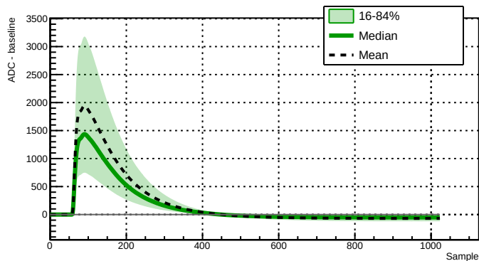
Run 039503 - Channel 2080 - 33111 waveforms
