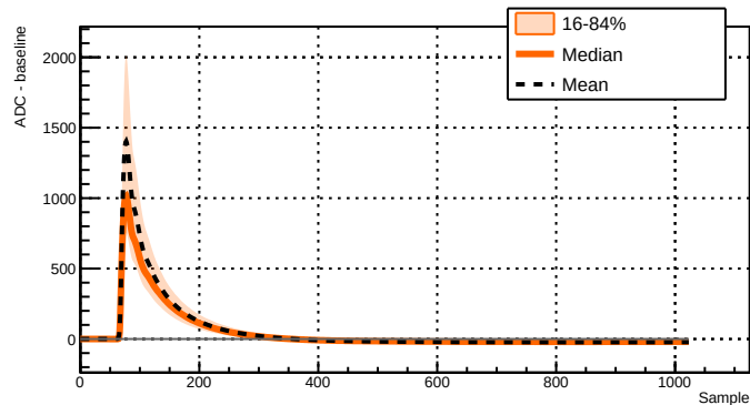
Run 039504 - Channel 2071 - 10295 waveforms
