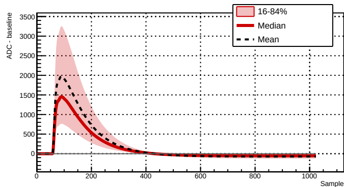
Run 039504 - Channel 2081 - 33348 waveforms
