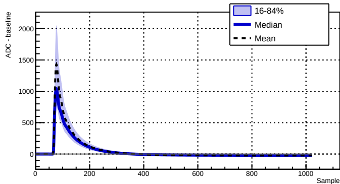
Run 039504 - Channel 2070 - 10445 waveforms
