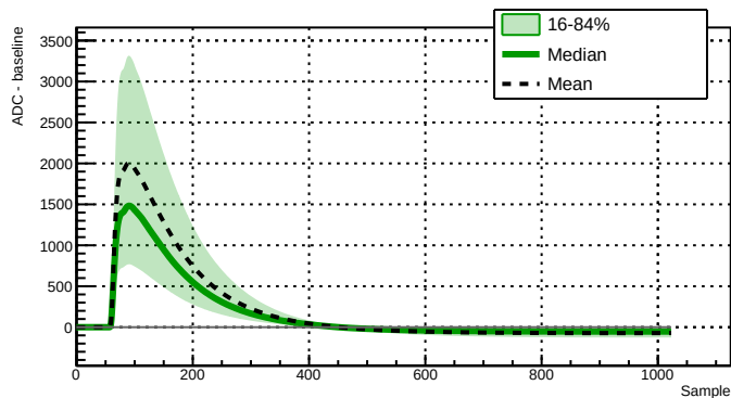
Run 039504 - Channel 2080 - 33869 waveforms
