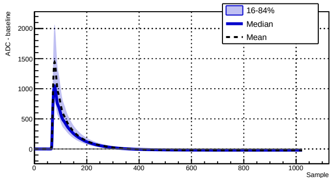
Run 039507 - Channel 2070 - 12106 waveforms
