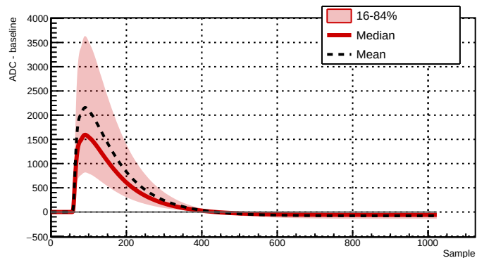
Run 039507 - Channel 2081 - 36620 waveforms
