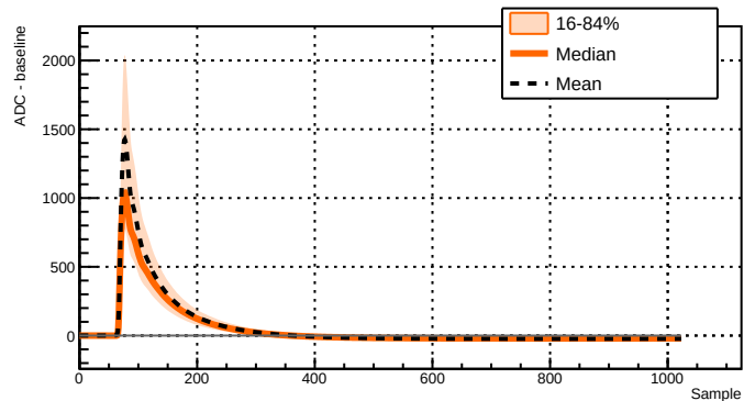
Run 039507 - Channel 2071 - 11739 waveforms
