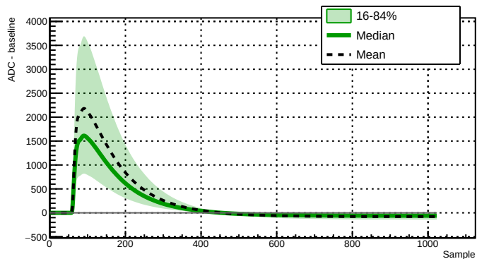
Run 039507 - Channel 2080 - 37270 waveforms
