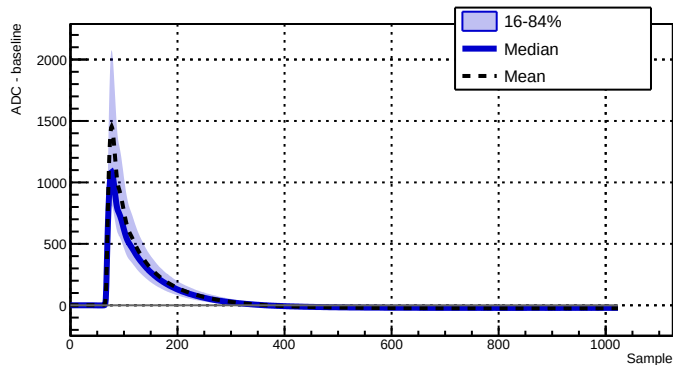
Run 039508 - Channel 2070 - 13012 waveforms
