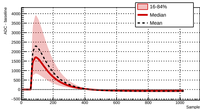
Run 039508 - Channel 2081 - 37963 waveforms
