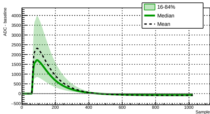
Run 039508 - Channel 2080 - 38428 waveforms
