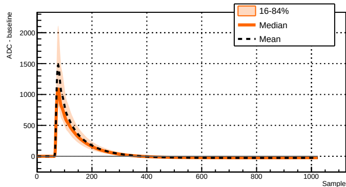
Run 039510 - Channel 2071 - 14002 waveforms
