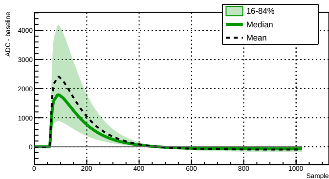
Run 039510 - Channel 2080 - 40981 waveforms
