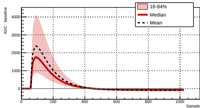
Run 039510 - Channel 2081 - 40487 waveforms
