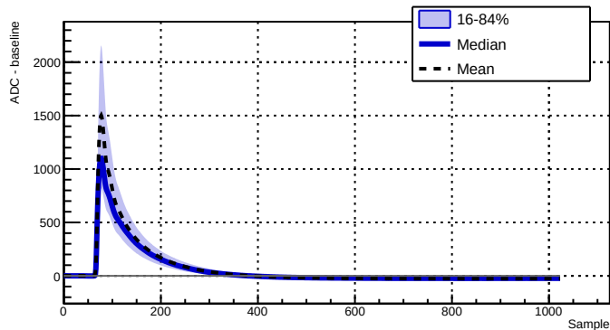
Run 039510 - Channel 2070 - 14308 waveforms
