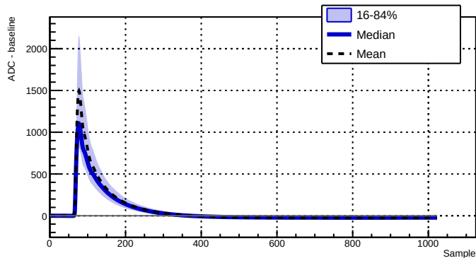
Run 039511 - Channel 2070 - 14001 waveforms
