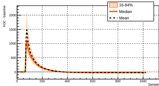
Run 039511 - Channel 2071 - 13727 waveforms
