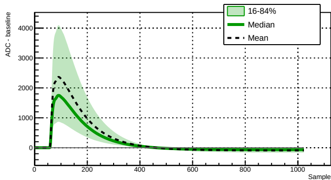
Run 039511 - Channel 2080 - 40448 waveforms
