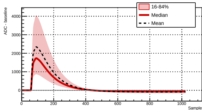
Run 039511 - Channel 2081 - 39984 waveforms
