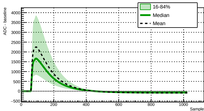
Run 039514 - Channel 2080 - 37265 waveforms
