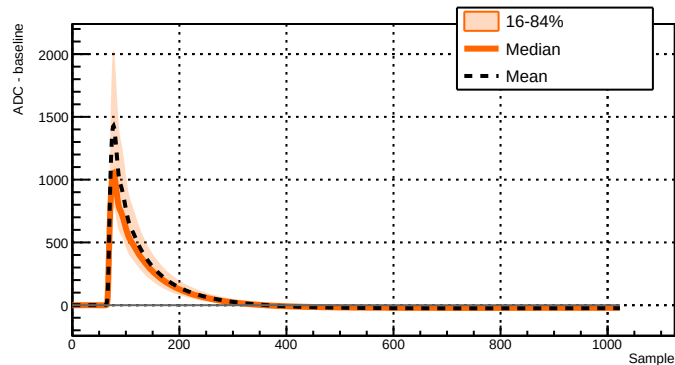
Run 039514 - Channel 2071 - 12172 waveforms
