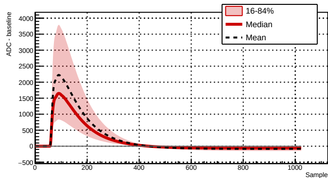
Run 039514 - Channel 2081 - 36695 waveforms
