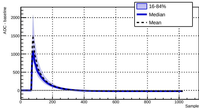
Run 039514 - Channel 2070 - 12450 waveforms
