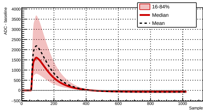
Run 039515 - Channel 2081 - 35031 waveforms
