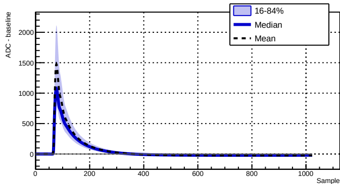
Run 039515 - Channel 2070 - 11810 waveforms
