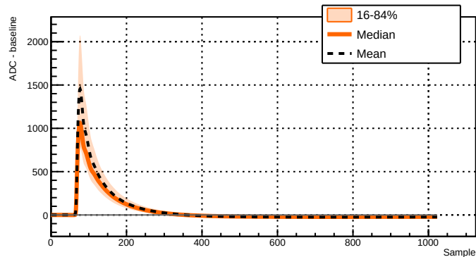
Run 039515 - Channel 2071 - 11464 waveforms
