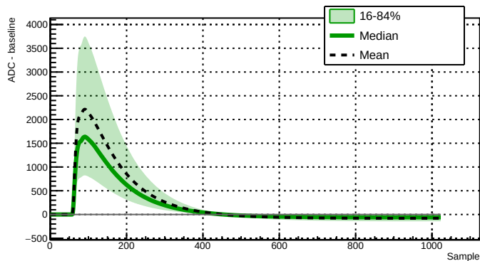
Run 039515 - Channel 2080 - 35498 waveforms
