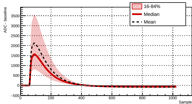
Run 039516 - Channel 2081 - 34248 waveforms
