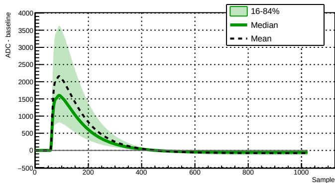
Run 039516 - Channel 2080 - 34603 waveforms
