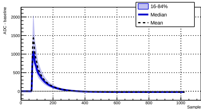
Run 039516 - Channel 2070 - 11338 waveforms
