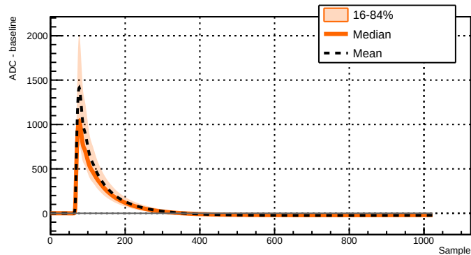
Run 039516 - Channel 2071 - 11074 waveforms
