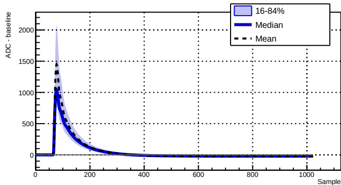
Run 039517 - Channel 2070 - 11168 waveforms
