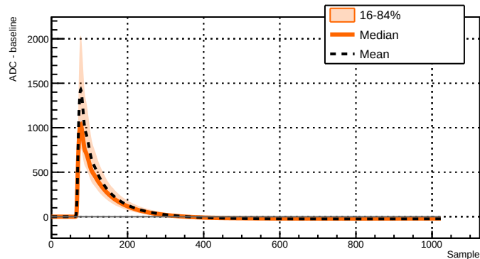
Run 039517 - Channel 2071 - 10890 waveforms
