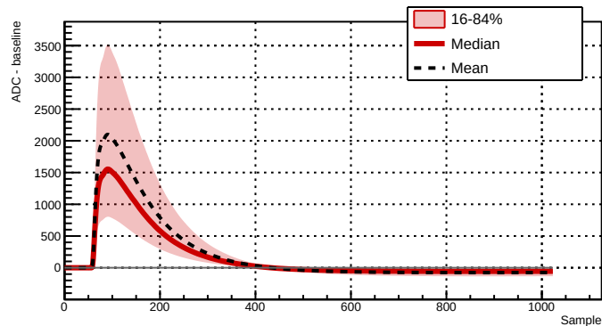
Run 039517 - Channel 2081 - 34274 waveforms
