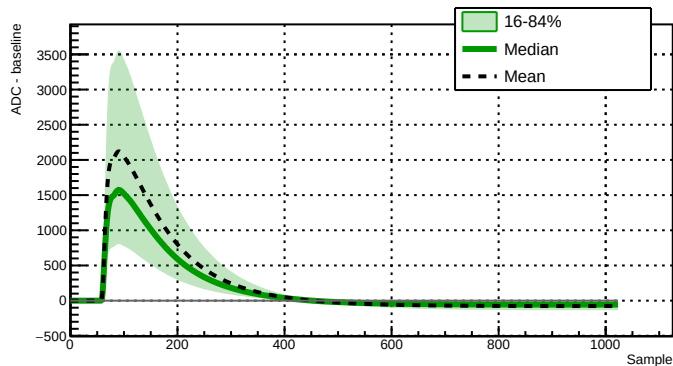
Run 039517 - Channel 2080 - 34696 waveforms
