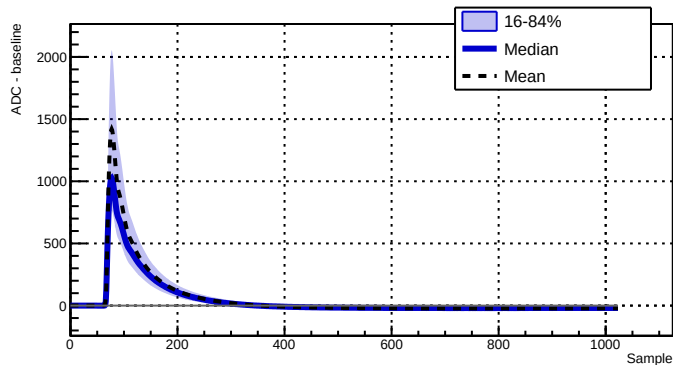
Run 039521 - Channel 2070 - 10056 waveforms
