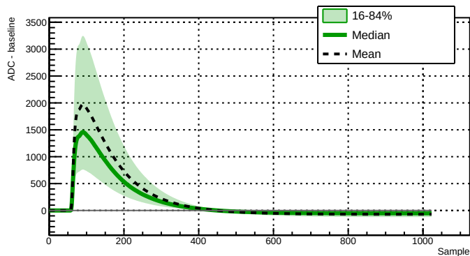
Run 039521 - Channel 2080 - 32571 waveforms
