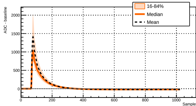
Run 039521 - Channel 2071 - 9835 waveforms
