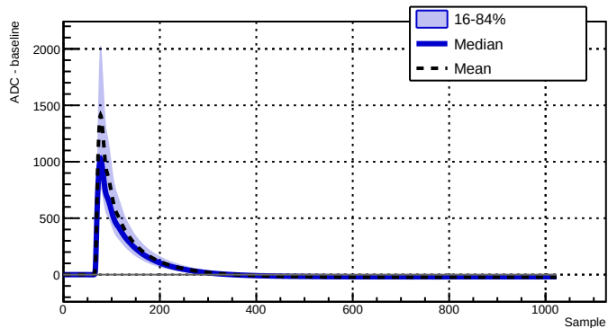
Run 039522 - Channel 2070 - 10007 waveforms
