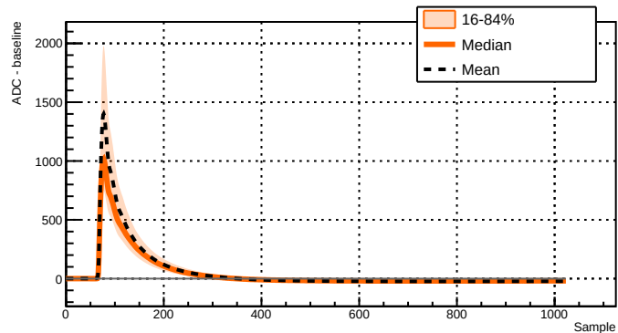
Run 039522 - Channel 2071 - 9694 waveforms
