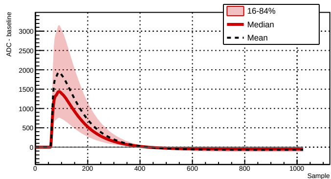
Run 039522 - Channel 2081 - 31838 waveforms
