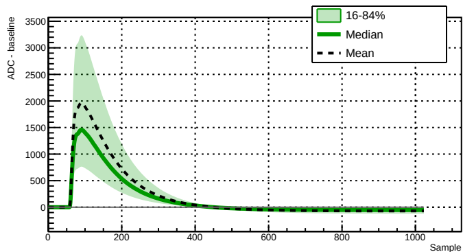
Run 039522 - Channel 2080 - 32280 waveforms
