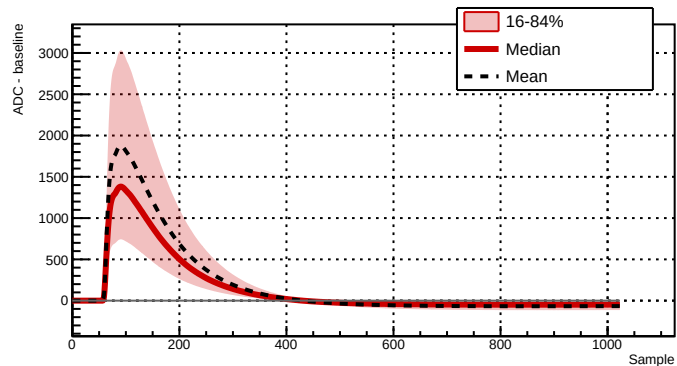
Run 039523 - Channel 2081 - 31132 waveforms
