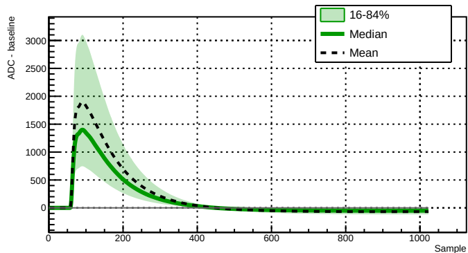
Run 039523 - Channel 2080 - 31566 waveforms
