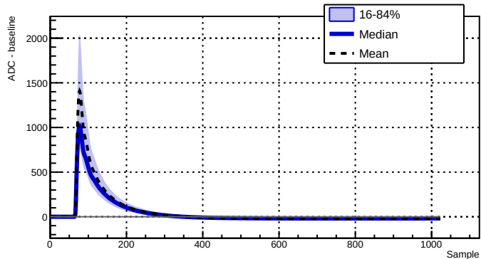
Run 039523 - Channel 2070 - 9588 waveforms
