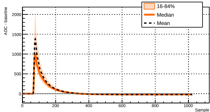
Run 039523 - Channel 2071 - 9383 waveforms
