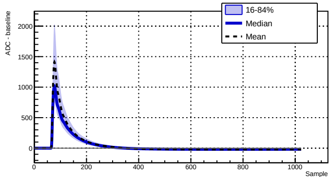
Run 039526 - Channel 2070 - 9078 waveforms
