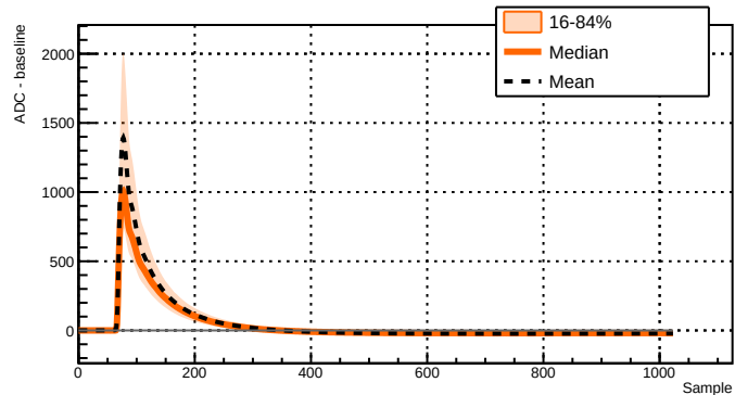
Run 039526 - Channel 2071 - 8855 waveforms
