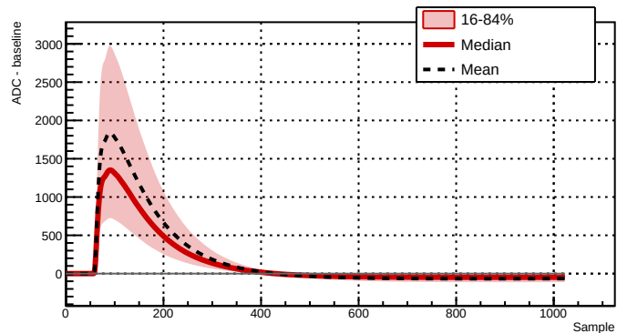
Run 039526 - Channel 2081 - 30172 waveforms
