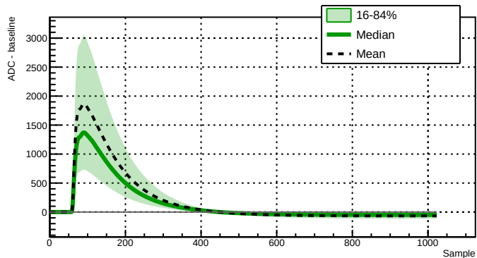
Run 039526 - Channel 2080 - 30652 waveforms
