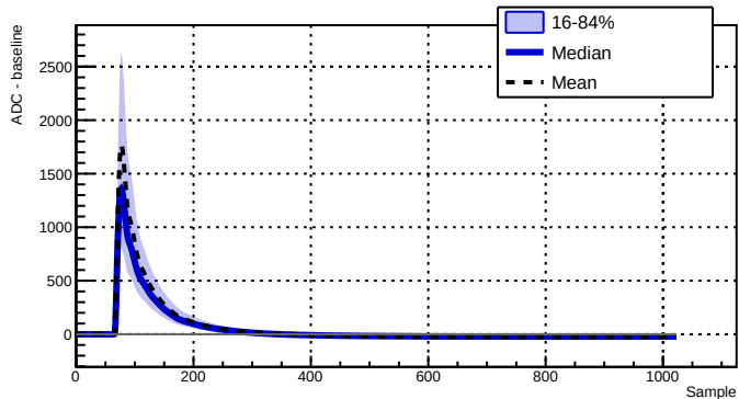
Run 039501 - Channel 2070 - 4848 waveforms
