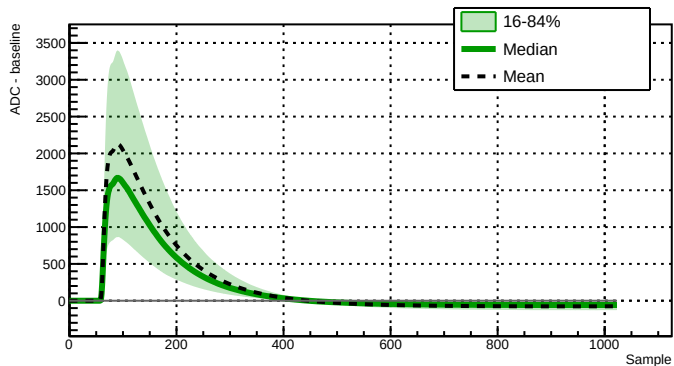
Run 039501 - Channel 2080 - 22132 waveforms
