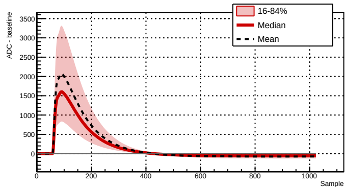
Run 039501 - Channel 2081 - 22868 waveforms
