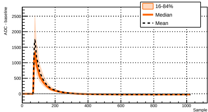
Run 039501 - Channel 2071 - 5045 waveforms
