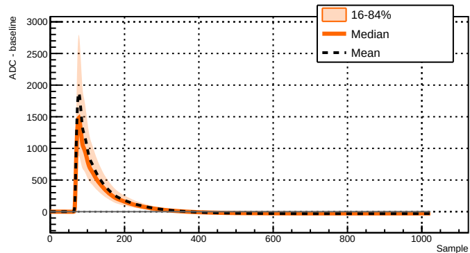
Run 039510 - Channel 2071 - 6947 waveforms
