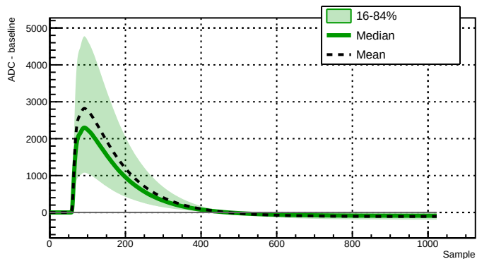
Run 039510 - Channel 2080 - 29765 waveforms
