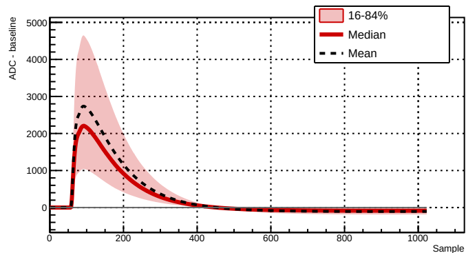
Run 039510 - Channel 2081 - 30058 waveforms
