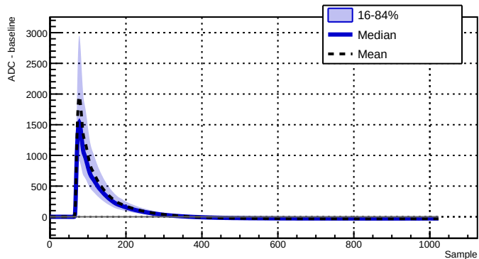
Run 039510 - Channel 2070 - 6471 waveforms
