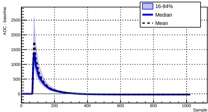
Run 039516 - Channel 2070 - 5755 waveforms
