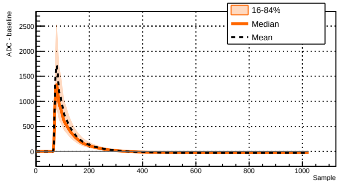
Run 039516 - Channel 2071 - 6115 waveforms
