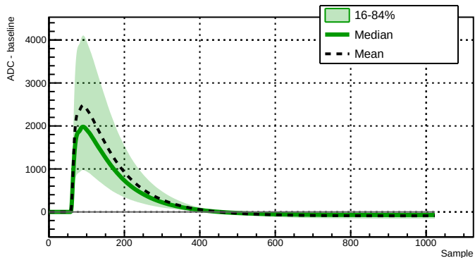
Run 039516 - Channel 2080 - 26052 waveforms
