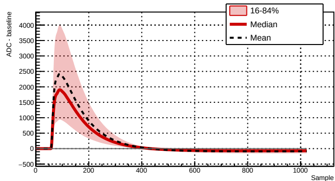
Run 039516 - Channel 2081 - 26410 waveforms
