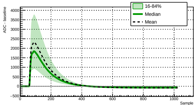
Run 039519 - Channel 2080 - 25038 waveforms
