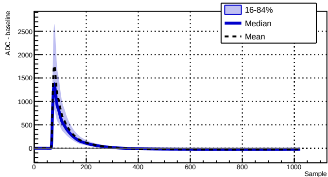
Run 039519 - Channel 2070 - 5511 waveforms
