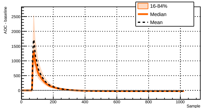
Run 039519 - Channel 2071 - 5785 waveforms
