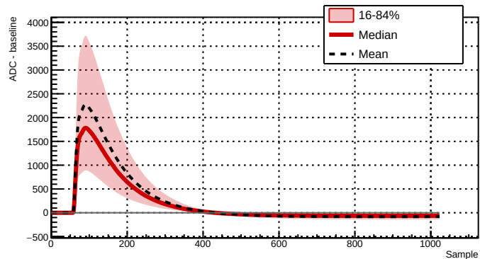
Run 039519 - Channel 2081 - 25461 waveforms
