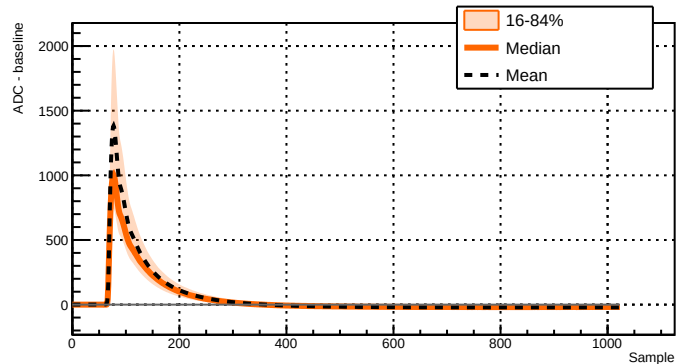
Run 039500 - Channel 2071 - 8694 waveforms
