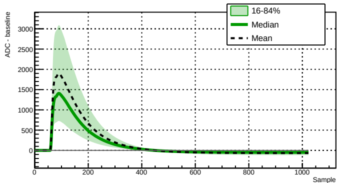
Run 039501 - Channel 2080 - 25721 waveforms
