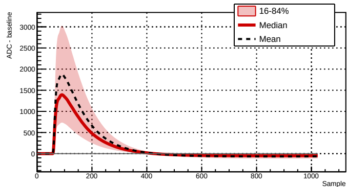
Run 039501 - Channel 2081 - 25862 waveforms
