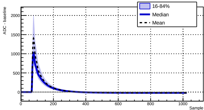
Run 039501 - Channel 2070 - 9400 waveforms
