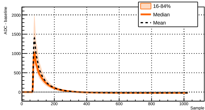
Run 039501 - Channel 2071 - 8975 waveforms
