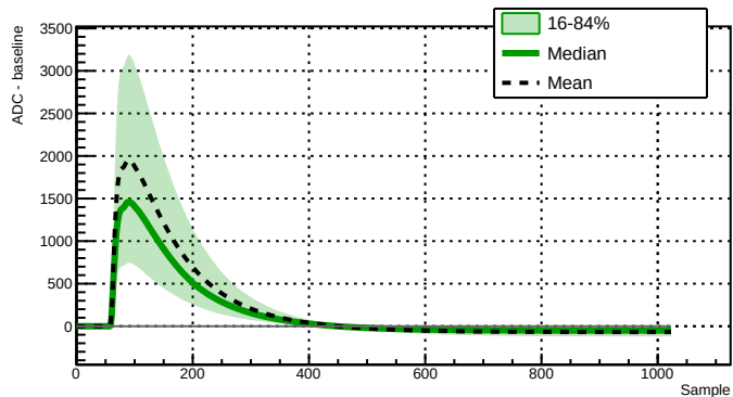
Run 039502 - Channel 2080 - 26124 waveforms
