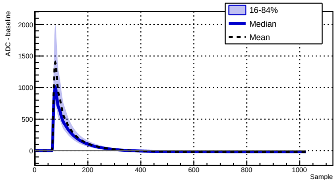
Run 039502 - Channel 2070 - 9949 waveforms
