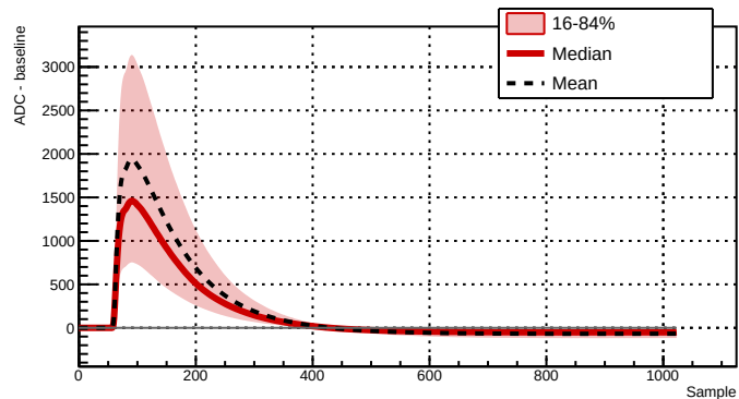
Run 039502 - Channel 2081 - 26223 waveforms
