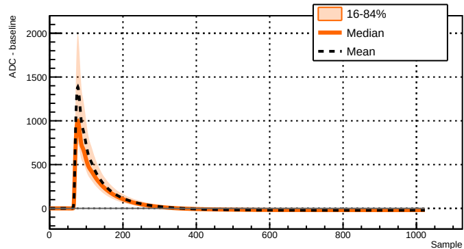
Run 039502 - Channel 2071 - 9592 waveforms
