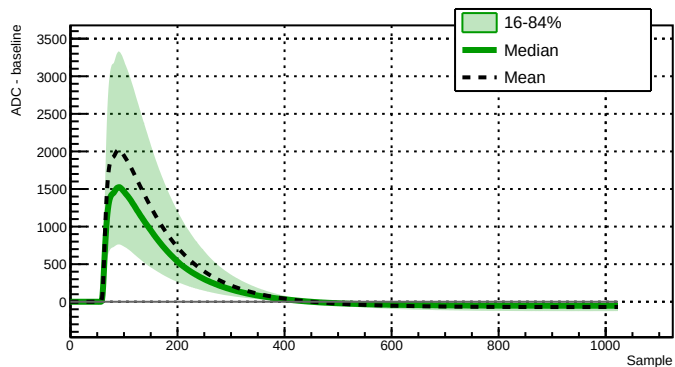
Run 039503 - Channel 2080 - 27274 waveforms
