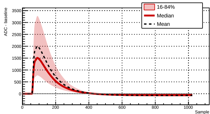
Run 039503 - Channel 2081 - 27288 waveforms
