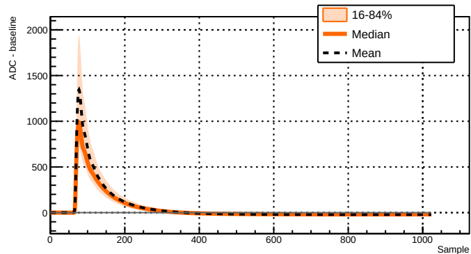
Run 039503 - Channel 2071 - 10518 waveforms
