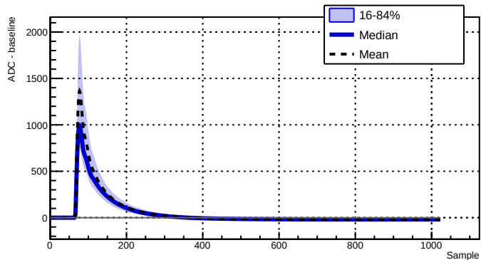
Run 039503 - Channel 2070 - 10859 waveforms
