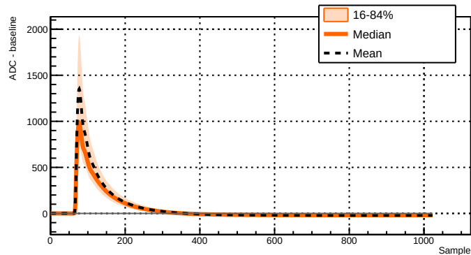
Run 039504 - Channel 2071 - 11059 waveforms
