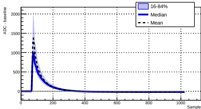
Run 039504 - Channel 2070 - 11408 waveforms
