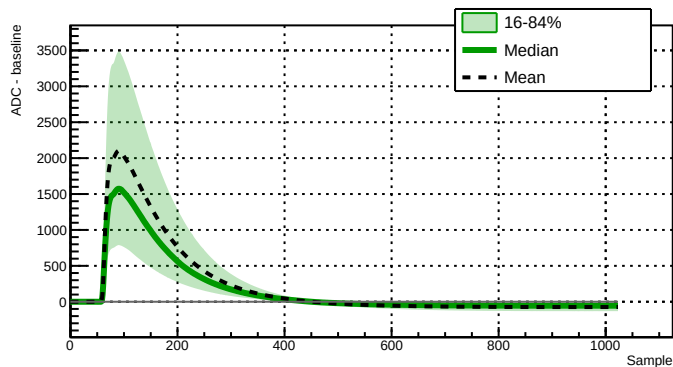
Run 039504 - Channel 2080 - 27535 waveforms
