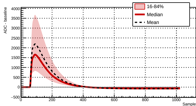
Run 039506 - Channel 2081 - 28928 waveforms
