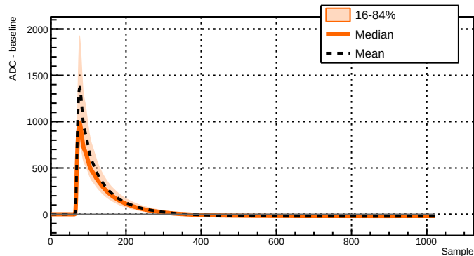
Run 039506 - Channel 2071 - 11873 waveforms
