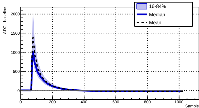
Run 039506 - Channel 2070 - 12285 waveforms
