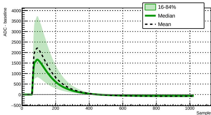
Run 039506 - Channel 2080 - 28515 waveforms
