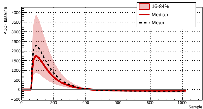
Run 039507 - Channel 2081 - 30112 waveforms
