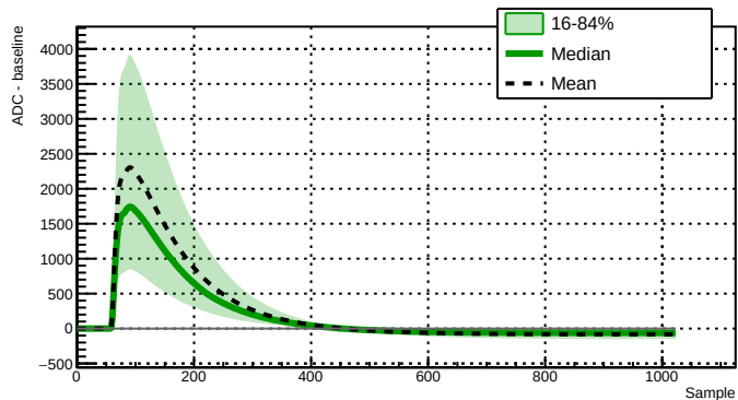
Run 039507 - Channel 2080 - 29715 waveforms
