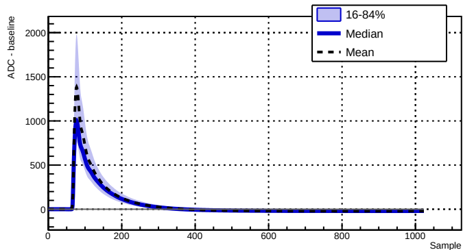
Run 039507 - Channel 2070 - 13079 waveforms
