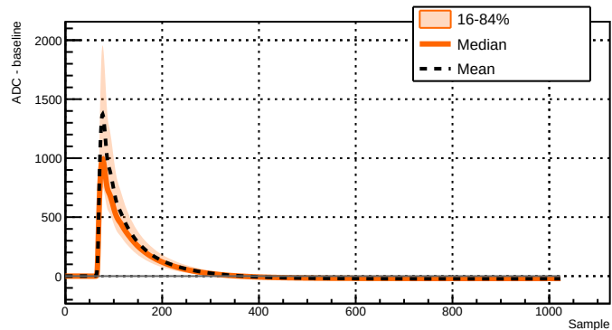
Run 039507 - Channel 2071 - 12610 waveforms
