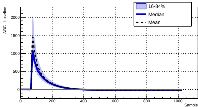
Run 039510 - Channel 2070 - 14723 waveforms
