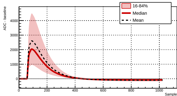
Run 039510 - Channel 2081 - 30159 waveforms
