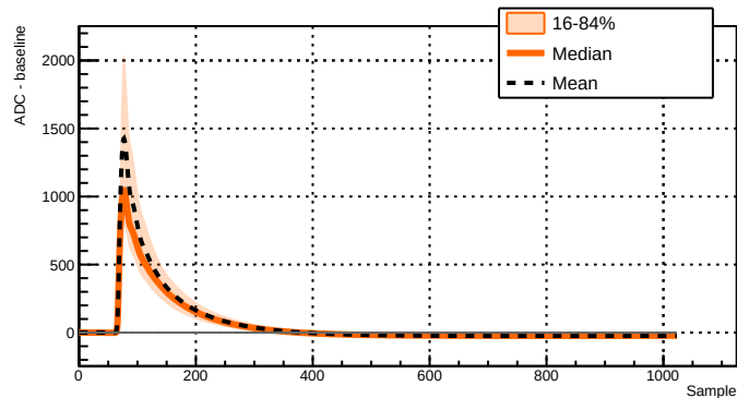
Run 039510 - Channel 2071 - 14323 waveforms
