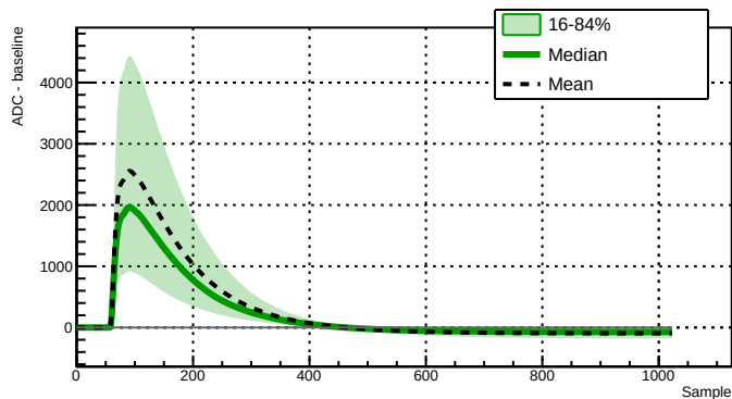
Run 039511 - Channel 2080 - 30912 waveforms
