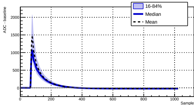
Run 039511 - Channel 2070 - 14613 waveforms
