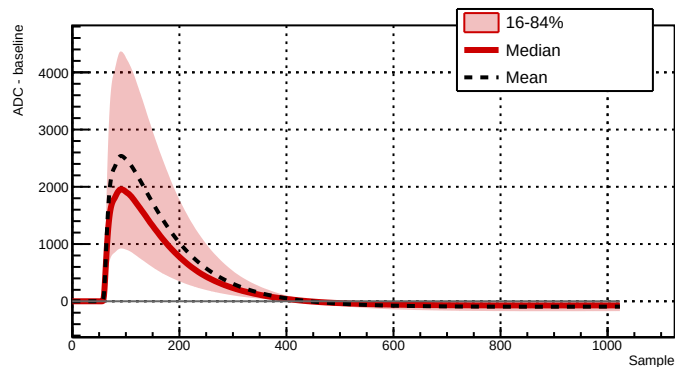
Run 039511 - Channel 2081 - 31468 waveforms
