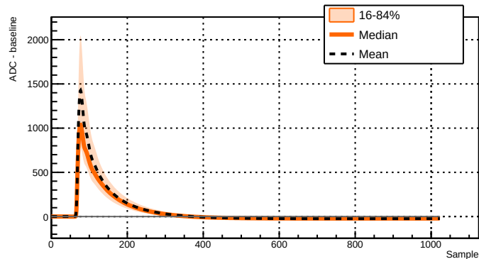
Run 039511 - Channel 2071 - 14200 waveforms
