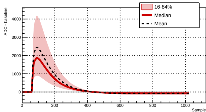
Run 039512 - Channel 2081 - 30760 waveforms
