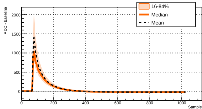
Run 039512 - Channel 2071 - 13572 waveforms
