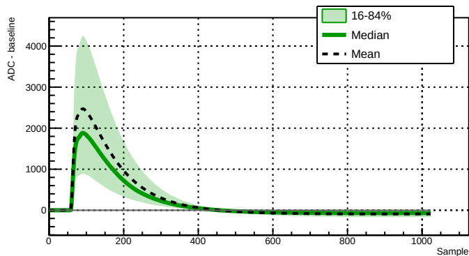
Run 039512 - Channel 2080 - 30174 waveforms
