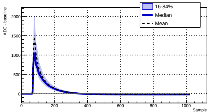
Run 039512 - Channel 2070 - 13940 waveforms
