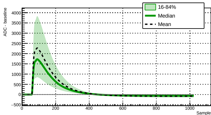
Run 039516 - Channel 2080 - 27994 waveforms
