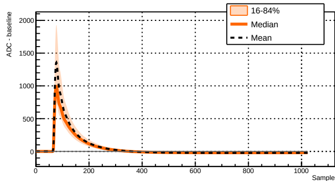
Run 039516 - Channel 2071 - 11942 waveforms
