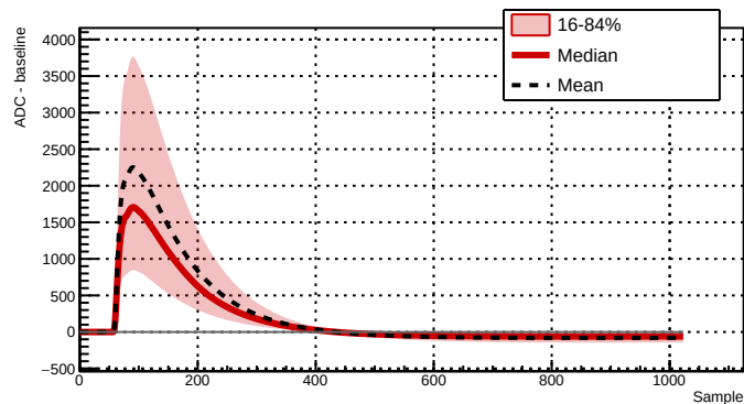
Run 039516 - Channel 2081 - 28261 waveforms
