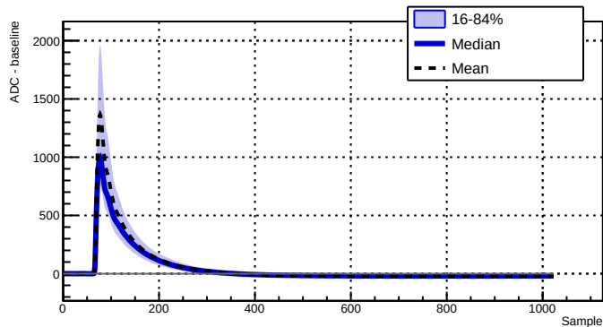
Run 039516 - Channel 2070 - 12303 waveforms
