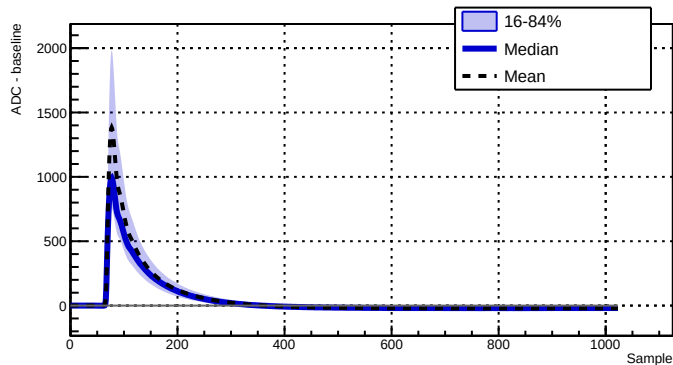
Run 039517 - Channel 2070 - 12104 waveforms
