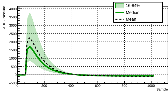
Run 039517 - Channel 2080 - 28153 waveforms
