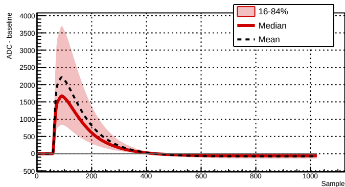
Run 039517 - Channel 2081 - 28595 waveforms
