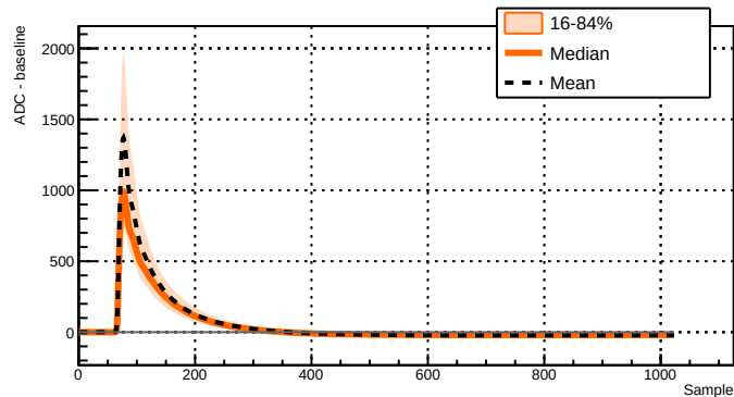
Run 039517 - Channel 2071 - 11744 waveforms
